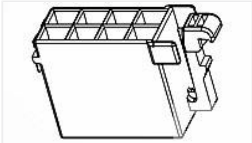
TE 产品编号1897122-3 8P JUNIOR-TIMER HSG,PART D2, ASS'Y
