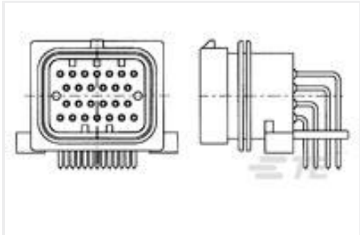
TE 产品编号9-6437287-8 SUPER SEAL 26POS CAP ASSY H AU
