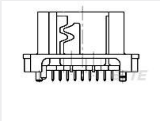
TE 产品编号967618-3 18pos MQS .63 header 180deg
