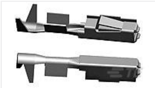
TE 产品编号5-963715-1 MQS0,63 Sn rec LL unseal. 0,5-0,75
