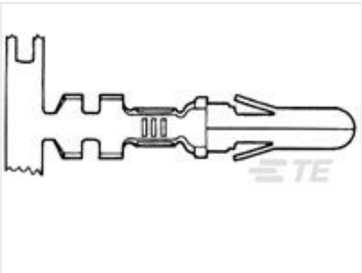
TE 产品编号350201-1 .140 DIA PIN 14-10 PTPBR
