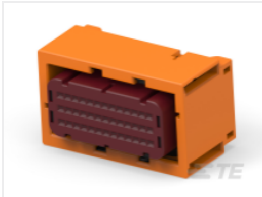
TE 产品编号2309307-4 GET 39P PLUG ASSY B1B9
