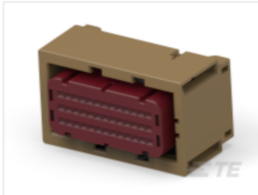
TE 产品编号5-2309307-9 GET 39P PLUG ASSY B2B4
