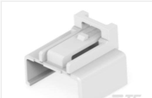
TE 产品编号2367917-1 TPA REC HSG,4POS,MQS
