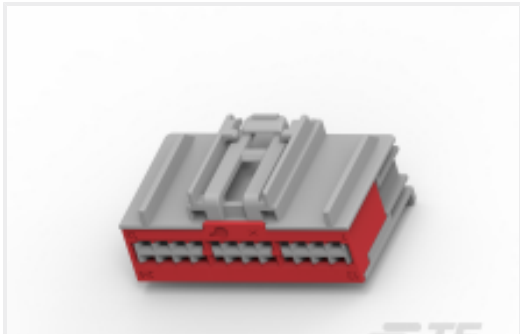
TE 产品编号1-1452839-5 24 POS FEMALE HSG ASSY
