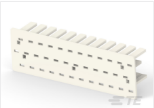
TE 产品编号344112-1 36W EMS.REC.ANTI-BACKOUT
