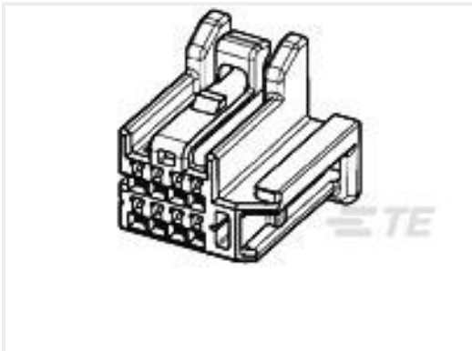
TE 产品编号 1318828-6 AIR BAG PLUG ASSY 8P
