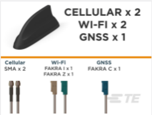
TE 产品编号L000423-08 5-Port,2x 5G/LTE,2x WiFi,GNSS,BLK
