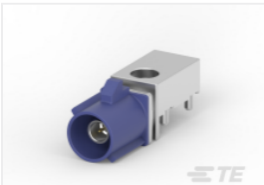
TE 产品编号5-2287906-3 FAKRA, 1 POS, EDGE MOUNT, 12 OCLOCK ASSY
