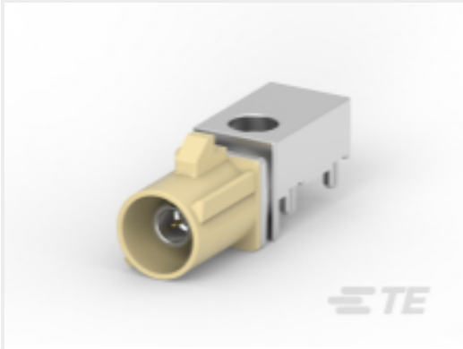
TE 产品编号5-2287906-9 FAKRA, 1 POS, EDGE MOUNT, 12 OCLOCK ASSY
