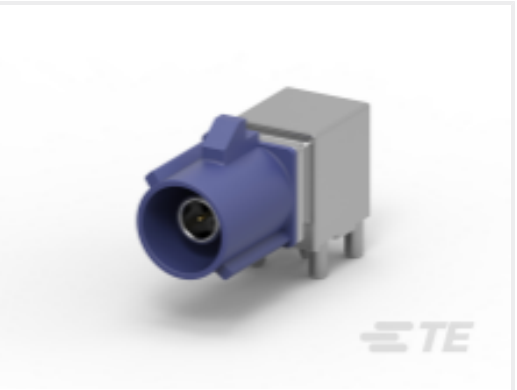
TE 产品编号2291392-3 MALE ASM, 1 POS, R/A, PCB, FAKRA
