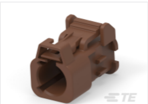
TE 产品编号1438893-6 PLUG HOUSING, 1 POSITION, 180 DEGREE, FA
