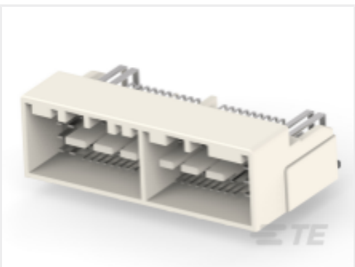
TE 产品编号1-2188692-1 020/060 73P HDR ASSY REFLOW
