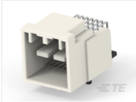
TE 产品编号2188695-1 020 21P HDR ASSY
