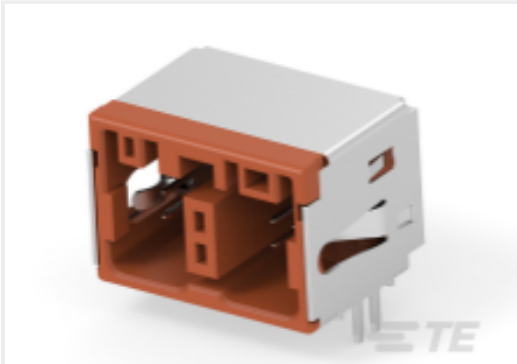
TE 产品编号2315739-4 8POS,0.50,HDR ASSY,180DEG,COD D, HSL
