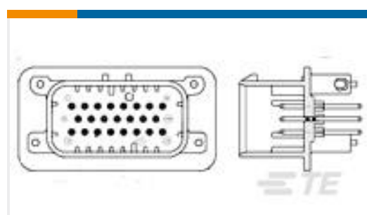
TE Part #1-776230-4 35POS,AMPSEAL,PIN HSG ASSY,SLD, COD 4
