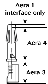
Female contact
