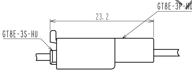
MATING CONFIGURATION
