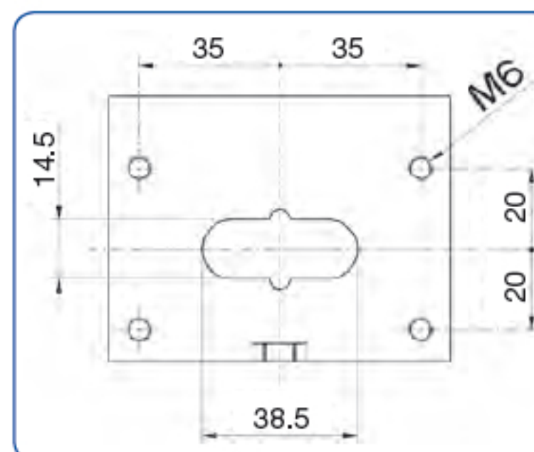
Header layout (code 1)
