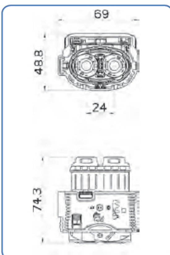
Female plug (code 1)
