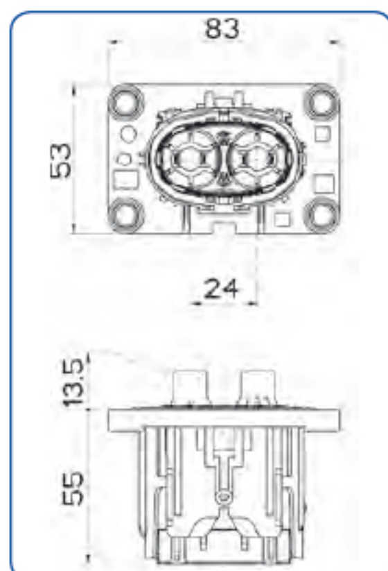
Male header (code 1)
