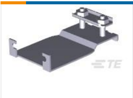
TE Part #201843-3 STRAIN RELIEF CLAMP (14) POS.
