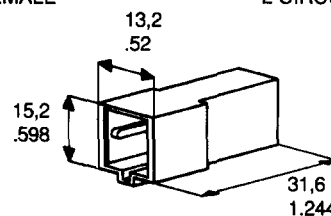
FEMALE 2 CIRCUITS
