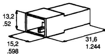
FEMALE 2 CIRCUITS
