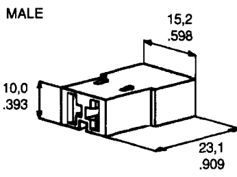
MALE
