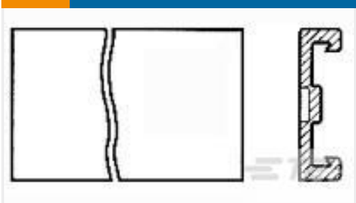
TE Part #640643-4 04P MTA156 COVER F/T
