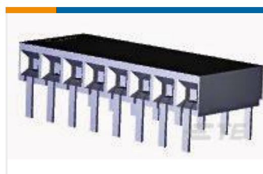
TE Part #5535676-7 08 MODII HORZ SR CE 100CL
