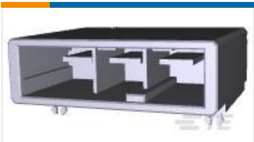
TE Part #1-353081-2 DYNAMIC D-5200 HDR H ASSY 3P
