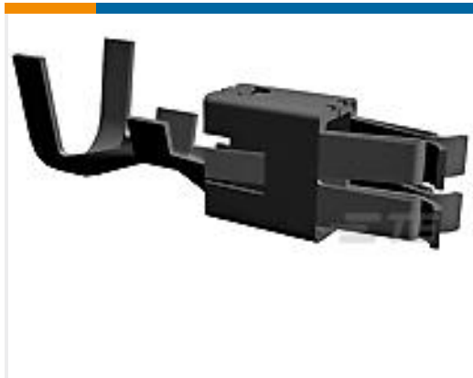
TE Part #962934-1 MPT REC 9.5 Contact SWS Sn
