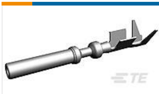
TE Part #3-1447221-4 S/S CONN REC CONTACT ASSEMBLY
