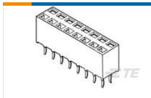
TE Part #2-215307-5 2X25P HV100 REC CON. TE, 7.0MM
