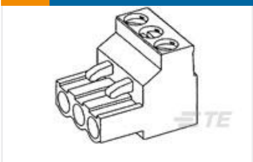
TE Part #796634-8 8 POS 5.08MM R/A PLUG,TRM BLK
