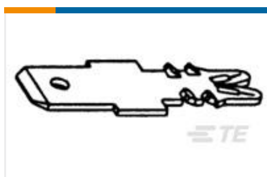
TE Part #1601035-1 131-082-000=TAB,187X032,STD5MZ
