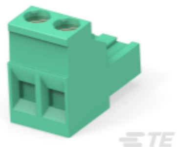
TE Part # 796640-2 2 POS 5.0 MM R/A PLUG,TRM BLK
