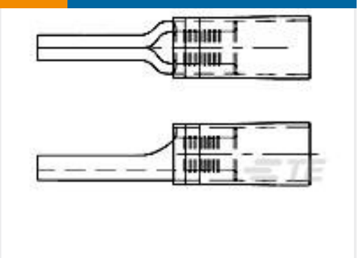
TE Part #2-696200-2 PIDG 12-10 WIRE PIN, TAPE
