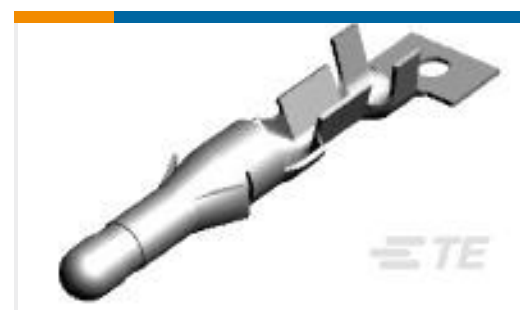
TE Part #770147-1 .093 CP&S PIN PTPBR LP 24-18
