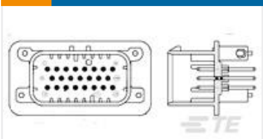
TE Part #776230-2 HEADER ASSY, 35 POS VERTICAL
