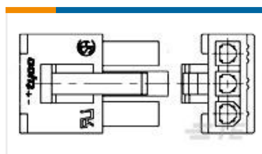
TE Part #521411-2 ULTRA POD: Flag, Receptacle Assembly, Tin Plated, .250 inch
