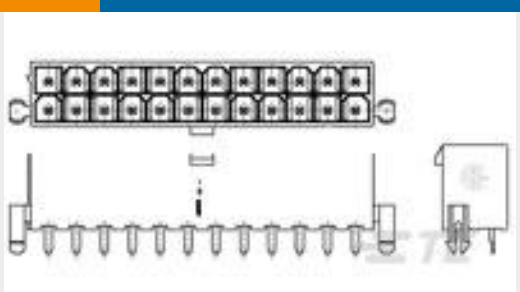
TE Part #2-1586039-0 20P VAL-U-LOK VRT HDR W/P V2
