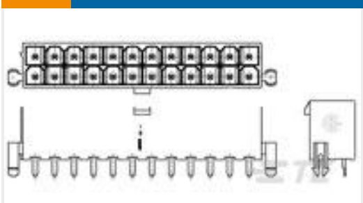
TE Part #1-1586039-8 18P VAL-U-LOK VRT HDR W/P V2
