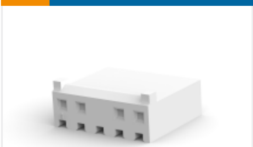
TE Part #640251-2 3.96mm Wire-to-board housing: receptacle, no mating alignment, SL 156
