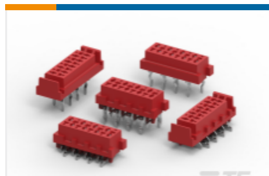
TE Part #8-338069-0 FEMALE-ON-BOARD CONNECTOR TOP ENTRY
