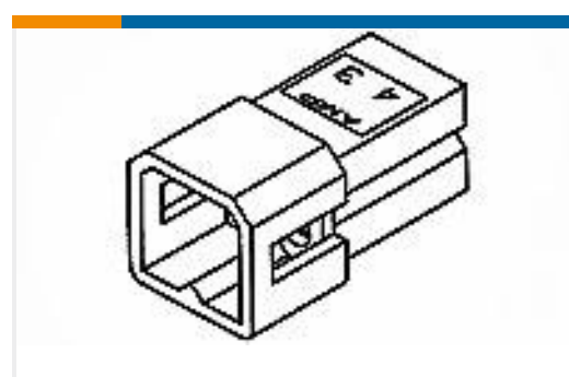
TE Part #770433-1 04P .062 COMM P&S PLUG
