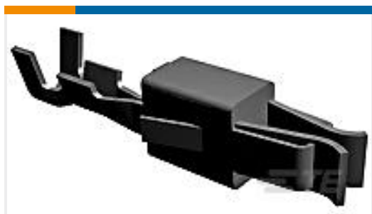
TE Part #927779-1 JPT REC 2.8 Contact SRC Sn (LP)
