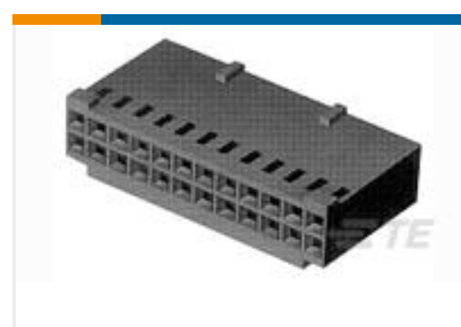
TE Part # 87977-8 20 MODIV HSG DR MRKD .100 POL
