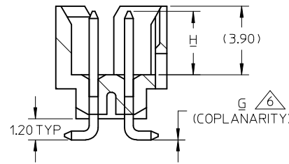
SECTION Z-Z
