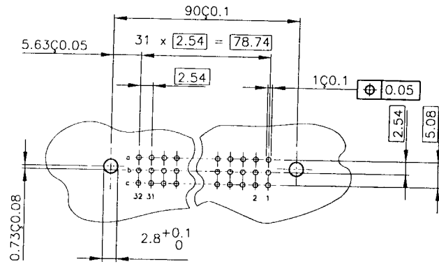
P.C. MOUNTING HOLE PATTERN
