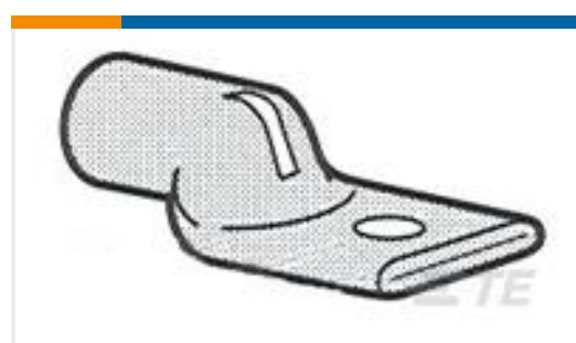
TE Part #325202 TERMINAL,AMPOWER 2 5/16
