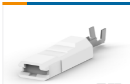
TE Part #520988-3 ULTRA-POD 250 ASSY REC 22-18 AWG TPBR
