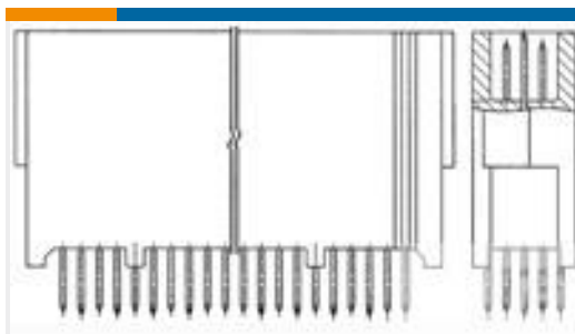
TE Part # 5536272-9 200,PLUG,VT,125,30AU
