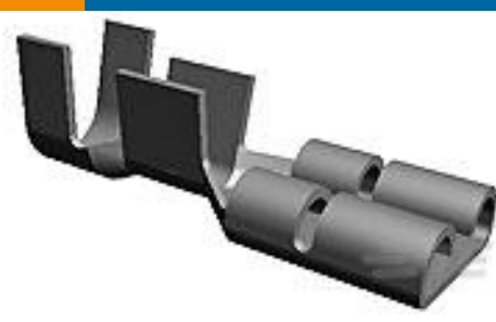
TE Part #63306-1 250 FASTON REC 18-14 AWG BR
