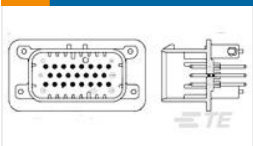
TE Part #776231-2 HEADER ASSY, 35 POS VERTICAL
