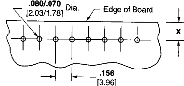
Recommended Mounting Hole Size for a .062 [1.57] Thk. PC Board
